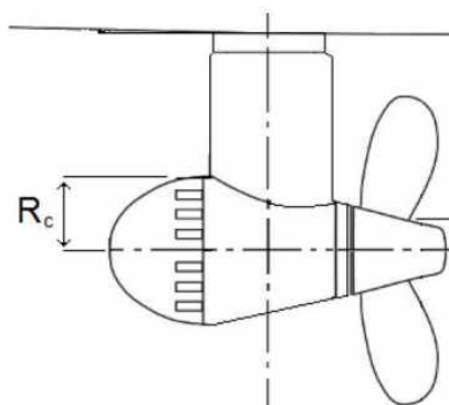
Fig 1.16 Dimensions used for R_c
