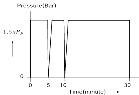
Fig 1.12.2 Test pressure/time curve
