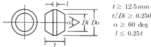
Fig 1.5.3 Double Beveled Disk Viewports
