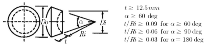
Fig 1.5.4 (a) Spherical Sector Viewports with Conical Edge
