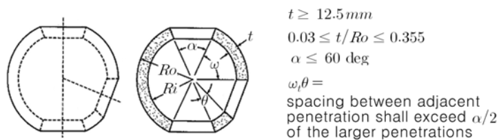
Fig 1.5.4 (c) NEMO Viewports
