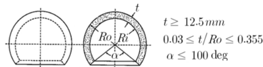
Fig 1.5.4 (b) Hyperhemispherical Viewports
