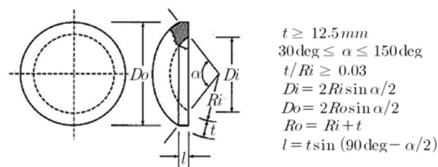
Fig 1.5.5 (a) Spherical Sector Viewports with Square Edge
