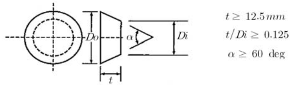
Fig 1.5.2 Conical Frustum Viewports
