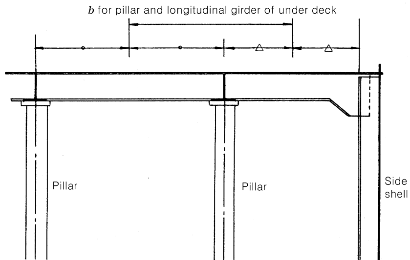
Fig 6.1 Measurement of S , b , l for pillar, and longitudinal and transverse girder
