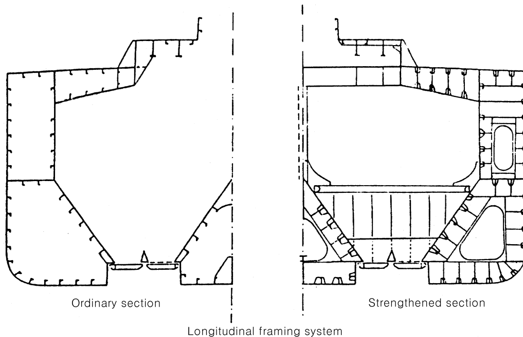
Fig 10.1 Hopper construction
