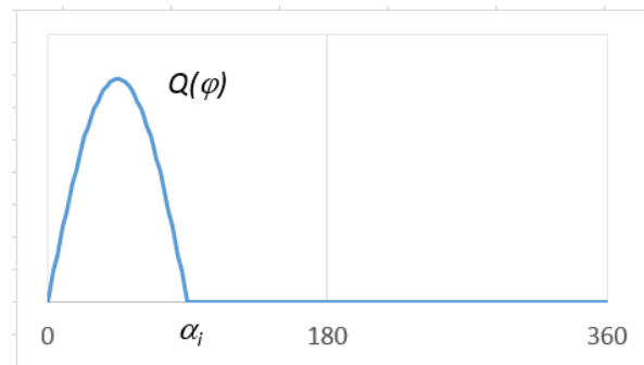
Schematic ice torque due to a single blade ice impact as a function of the propeller rotation angle
