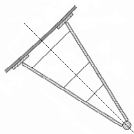
Fig 1.6 An example of typical type bilge keel construction
