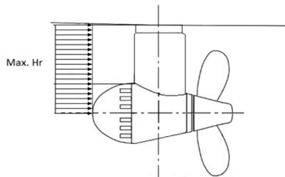
Fig 1.16 Schematic figure showing the reduction of the contact area by the maximum ridge thickness
