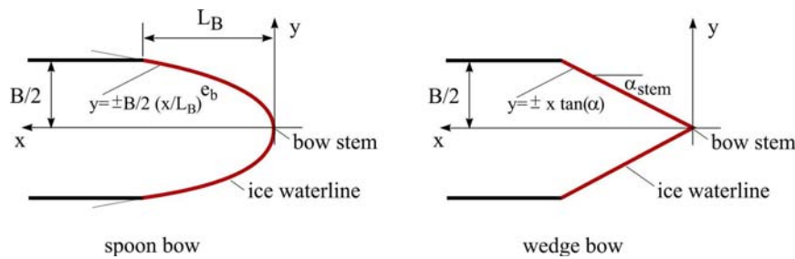
Fig 2.7 Bow shape definition
