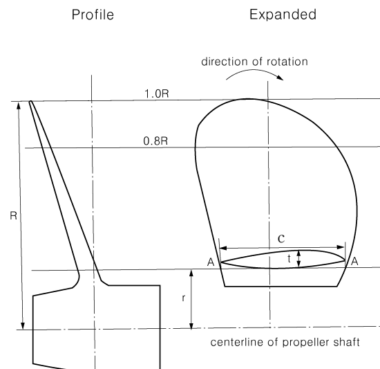
Fig 1.11 Dimension of propeller section for calculation of blade failure load
