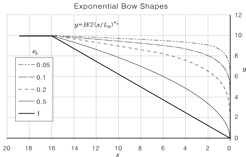
Fig 2.8 Illustration of e_b effect on the bow shape for B = 20 and L_B = 16
