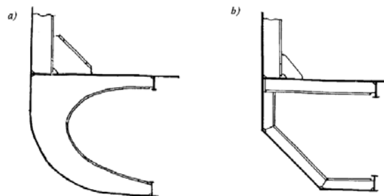
Fig 3.9 a - lighted margin bracket, b - system of stiffeners
