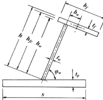
Fig 2.4 Stiffener geometry
