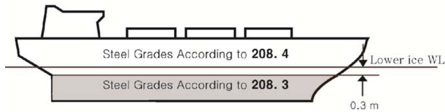
Fig 2.6 Steel grade requirements for submerged and weather exposed shell plating
