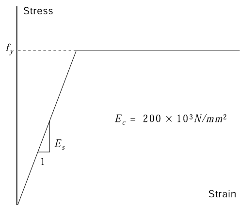
Fig. 3.6.2 Stress-Strain Relation for Non-Prestressed Steel in Uniaxial Tension
