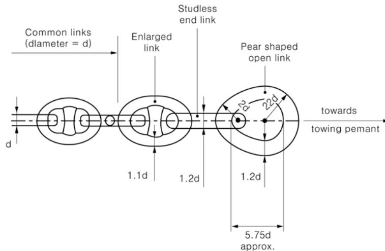
Fig 4.8.10 Typical outboard chafing chain end
