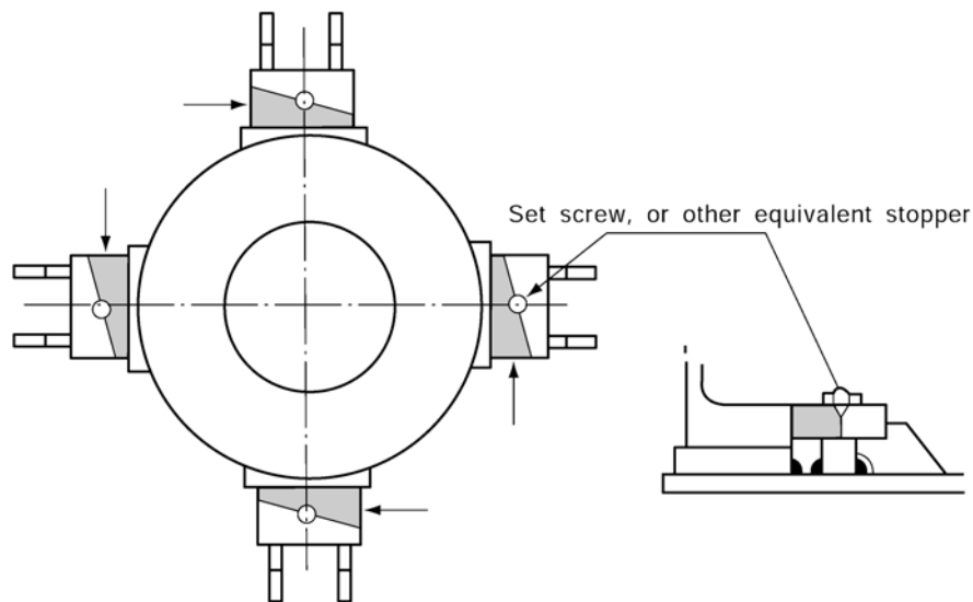
Fig 4.1.15 Fixing arrangement of rudder carrier on deck
