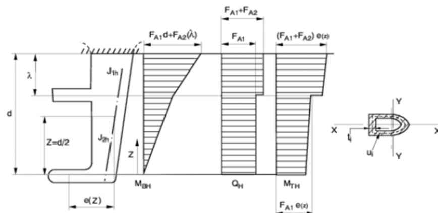
Fig 4.1.8 Rudder horn
