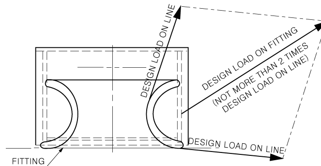
Fig 4.10.1 Application of design load
