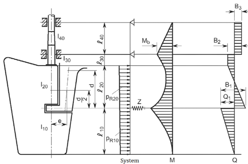
Fig 4.1.5 Type D rudder (Semi spade rudder with one elastic support)
