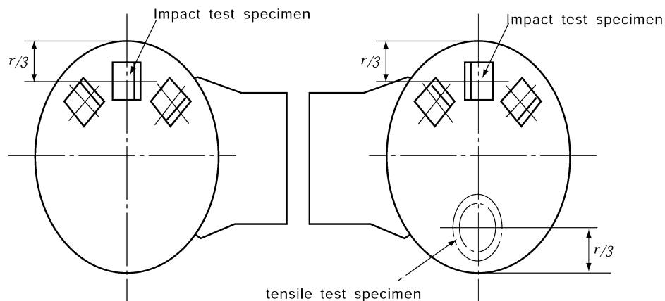
Fig 4.8.12 Location for sampling test specimens for links of offshore chains
