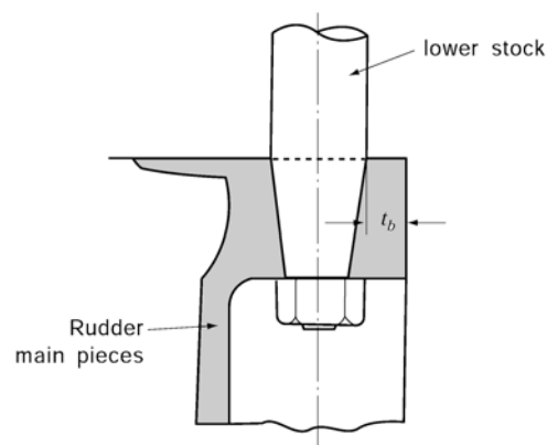
Fig 4.1.12 Coupling between rudder lower stock and rudder main pieces
