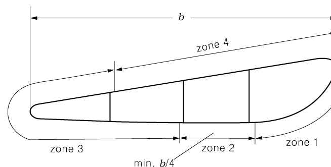
Fig 4.1.6 Propeller zone
