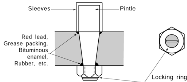
Fig 4.1.13 Locking device and preventing device of corrosion of pintle nut
