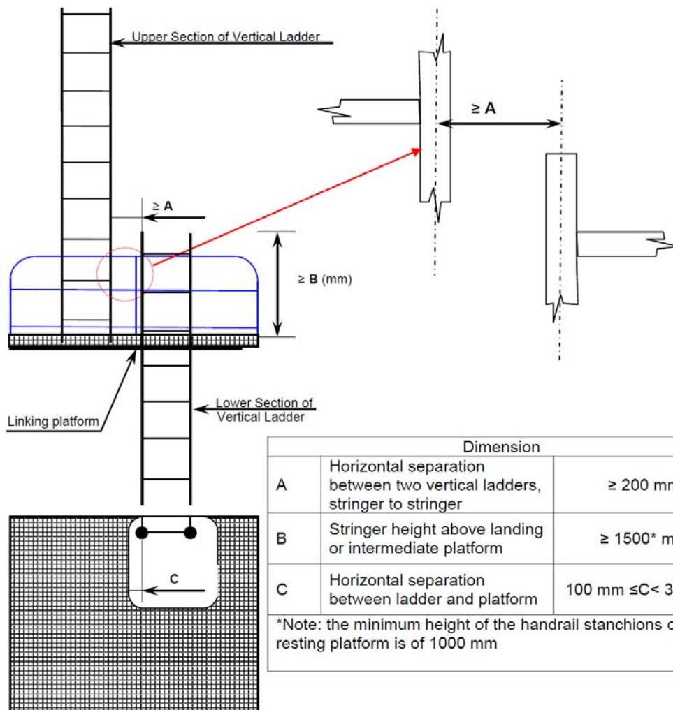
Vertical Ladder - Ladder through the linking platform
