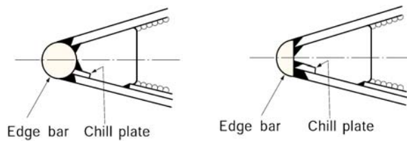
Fig 4.1.11 Structure of end part of rudder
